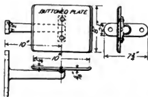
Figs. 3309-3311. Headlight Slip on Smokebox Front.
